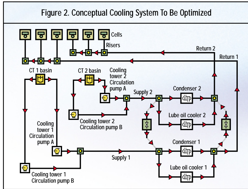
For the cooling system shown here, the design requirement is to supply 15,000 gpm to each condenser and 700 gpm to each lube oil cooler.
