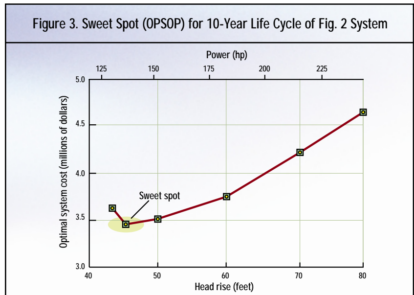
Using cost data, the piping system optimizer can identify the sweet spot among all potential designs.
