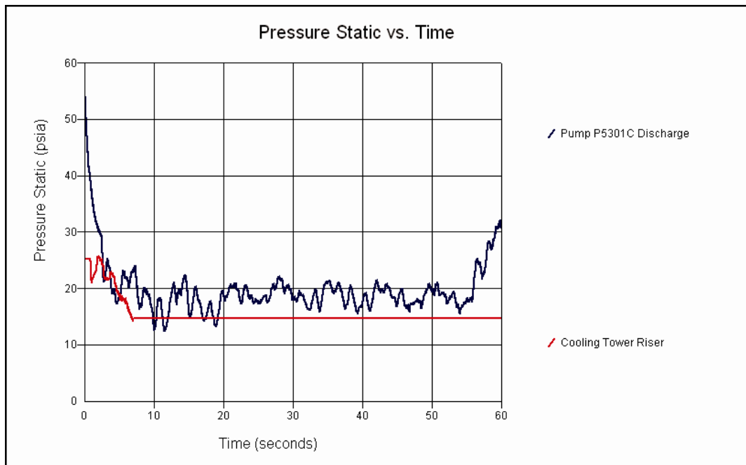
Pressure vs. time graph at pump discharge and inlet of cooling tower riser after pump trip
