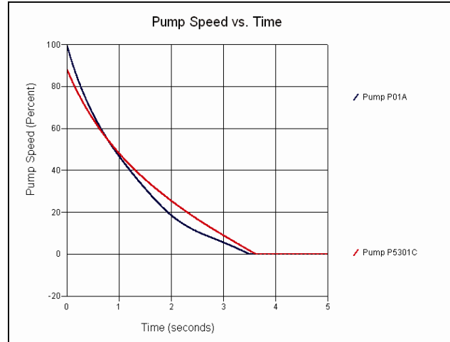
Pump speed vs. time graph for one of the existing circulating pumps and one of the new booster pumps after tripping
